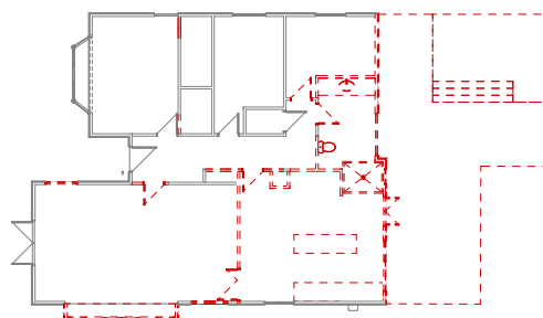
EXISTING/DEMOLITION PLAN
