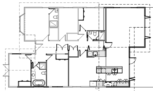
PROPOSED PLAN
